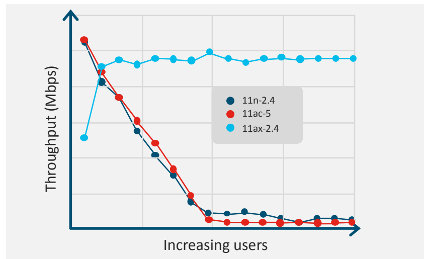
Figure 1 – The ability of Wi-Fi 6 to improve capacity is clearly revealed in this chart of test results. Unlike previous generations, per-user throughput is maintained even as traffic volumes grow. Source: Cisco Systems.
