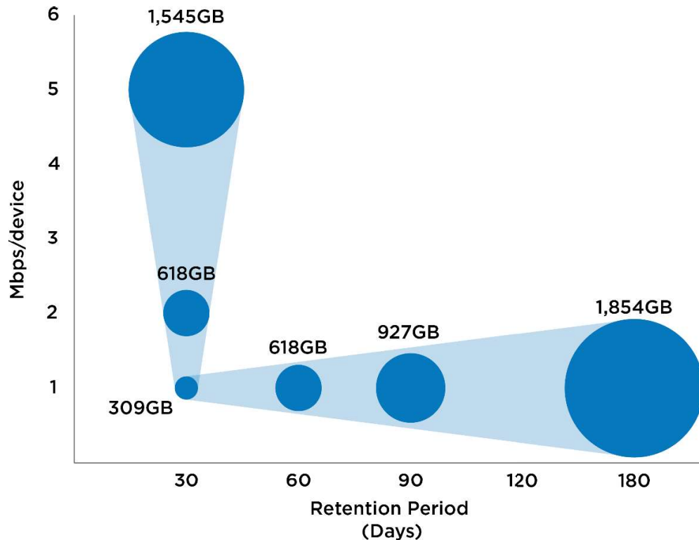
Figure 2) Simple sizing with DE Series: storage required for a single camera with a given throughput and retention period.
