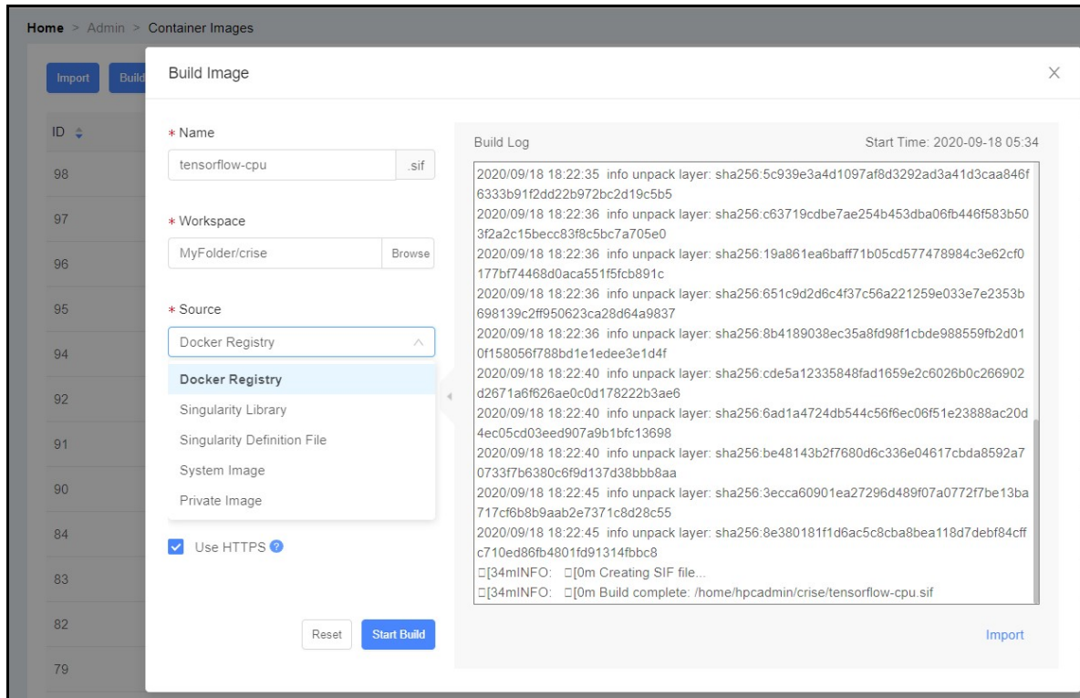
Figure 25. Singularity container building within LiCO
