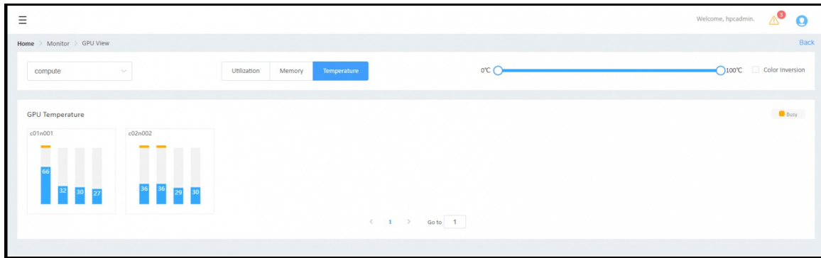
Figure 32. LiCO HPC/AI GPU View dashboard
