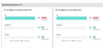
FIGURE 6. Resource Planner
