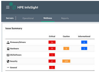
FIGURE 3. Wellness dashboard
