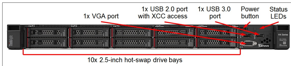
Figure 2. ThinkAgile HX3320 Appliance for SAP HANA front view
