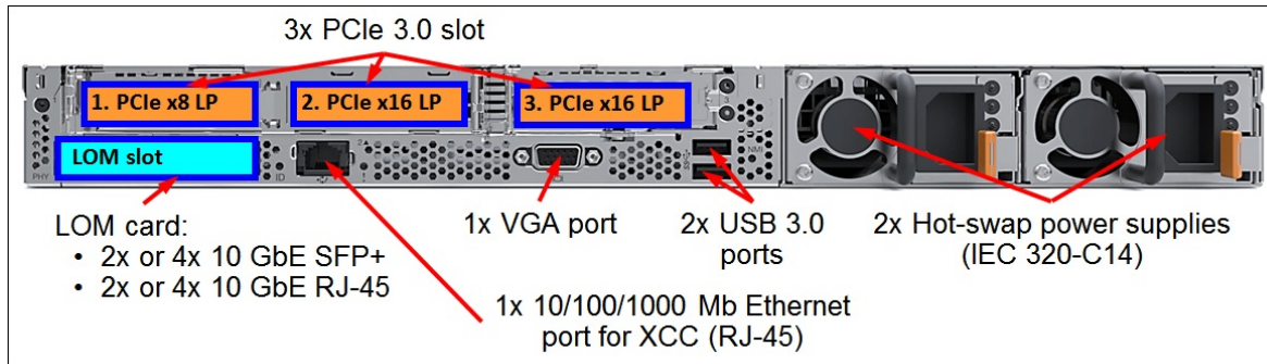
Figure 3. ThinkAgile HX3320 Appliance for SAP HANA 10-drive bay rear view
