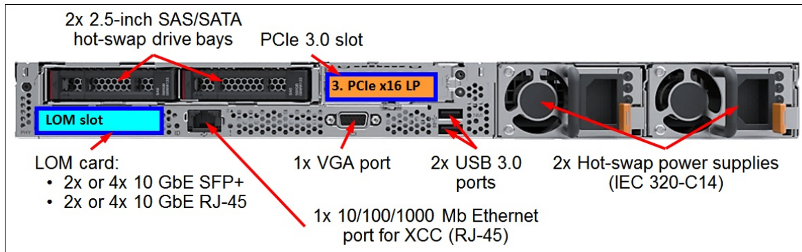
Figure 4. ThinkAgile HX3320 Appliance for SAP HANA 12-drive bay rear view
