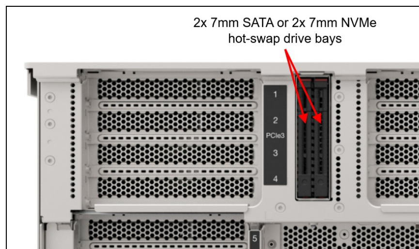
Figure 11. 7mm drive bays
