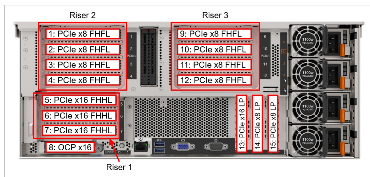
Figure 12. SR860 V2 slot numbering
