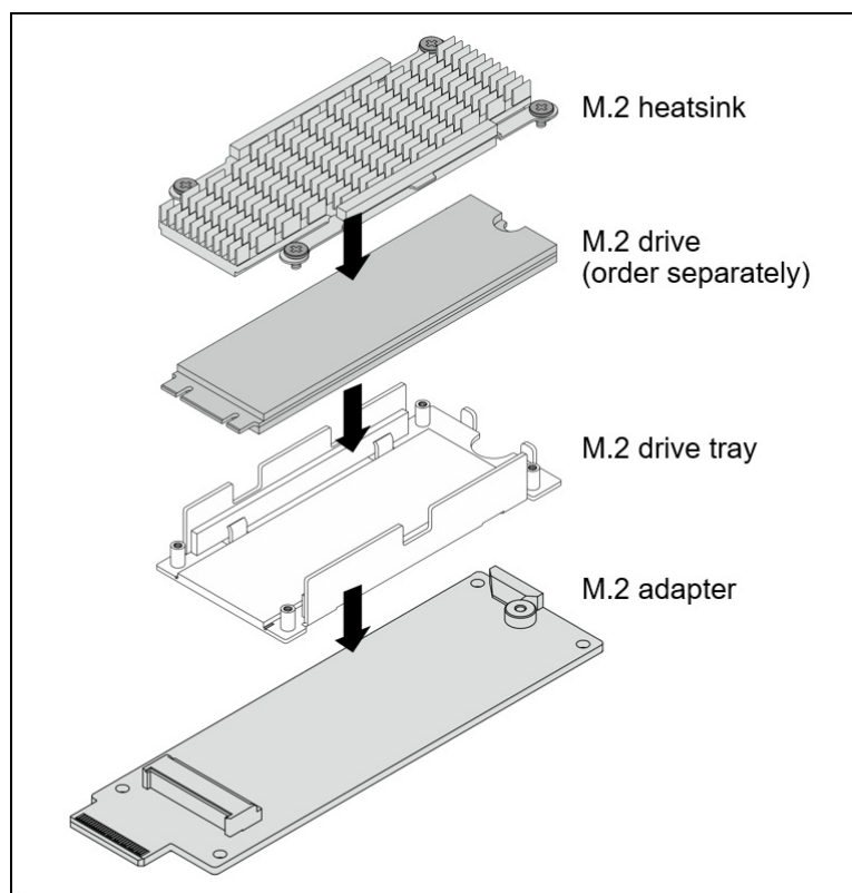
Figure 15. Components of the ThinkSystem V4 Hot Swap M.2 SATA/NVMe Drive Assembly Kit
