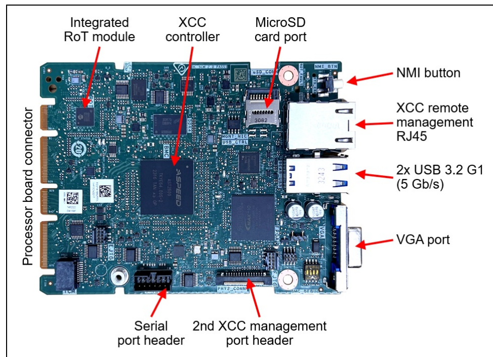
Figure 25. System I/O Board
