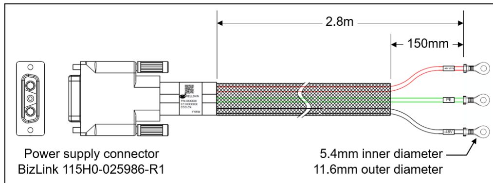
Figure 23. -48V DC power cord
