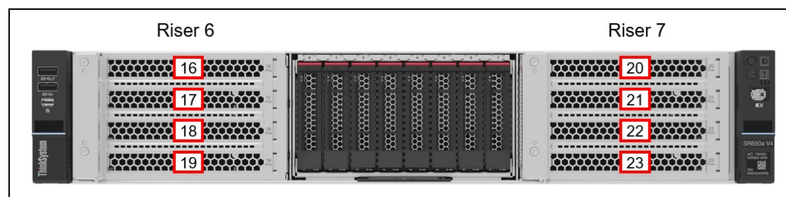
Figure 16. SR650a V4 front slots
