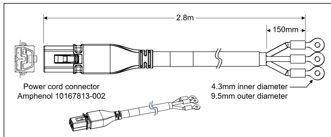
Figure 24. HVDC power cord
