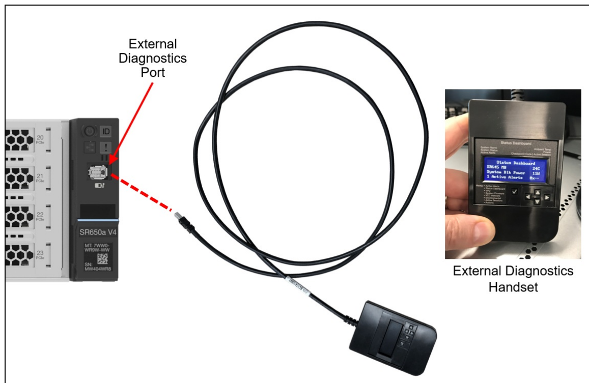
Figure 27. External Diagnostics Handset
