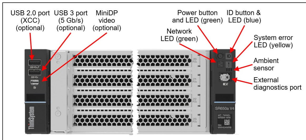
Figure 26. Front operator controls are on the left and right side of the server
